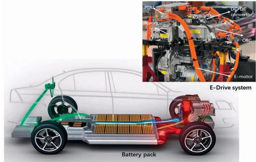
Fig. 1. Key components of the high voltage drive train system of a Chevrolet Bolt (© DSM)
