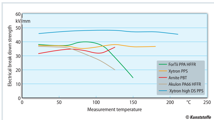
Fig. 7. Electric breakdown strength before aging at elevated temperatures. Most polymers show a decline in breakdown strength at rising temperatures (source: DSM)
