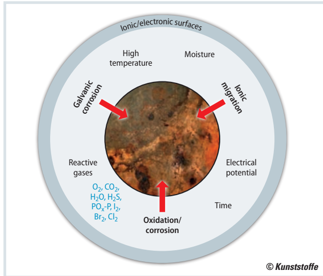
Fig. 3. Terminal corrosion caused by outgassed heat stabilizers or migration of other ionic impurities in the plastic (source: DSM)
