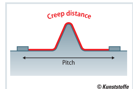
Fig. 5. The creep distance is often deliberately increased to prevent the flow of current between two contacts
