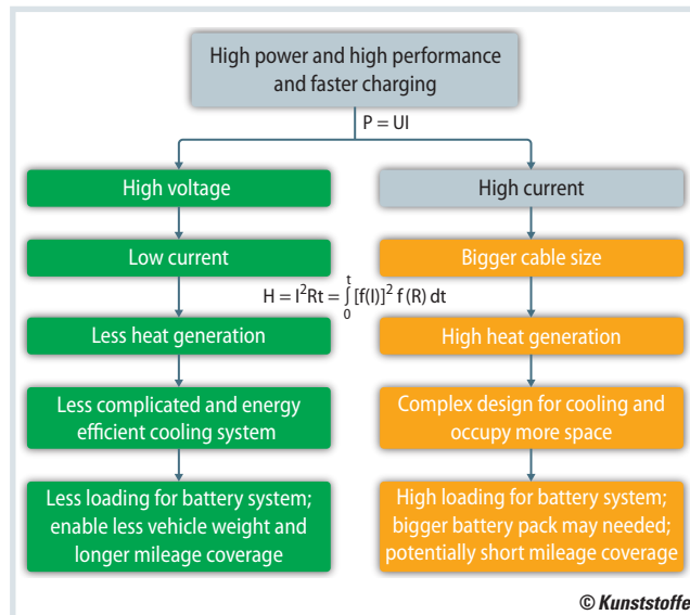
Fig. 4. In order to increase the battery performance, it is usually more advisable to increase the voltage rather than the current
