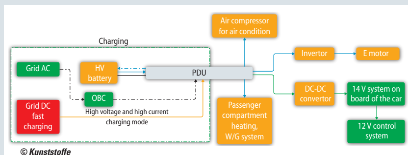
Functional diagram of the powertrain in a battery electric vehicle. Electrification adds further components (source: DSM)
