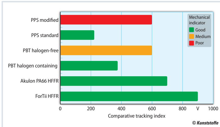
Fig. 6. Comparison of different polymer classes by tracking resistance. Colors indicate respective mechanical strength (source: DSM)
