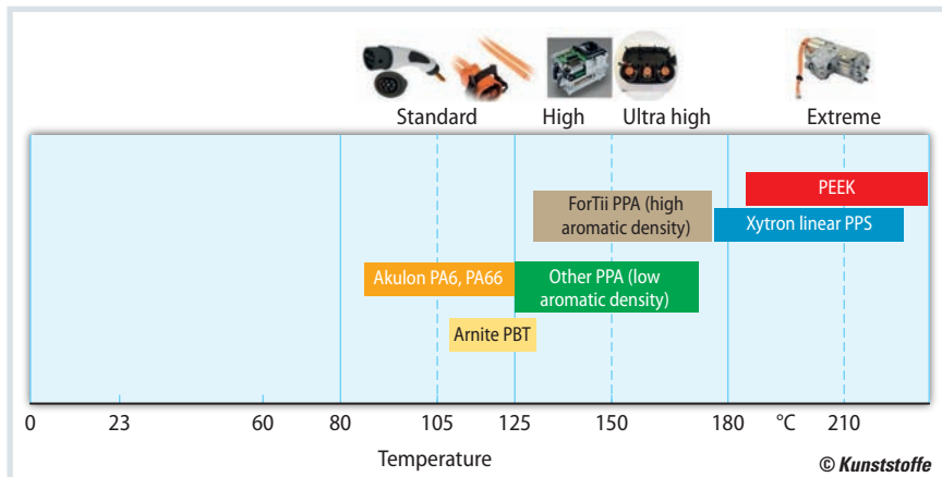
Fig. 9. DSM high-voltage material portfolio for high operating temperatures. Different materials are recommended depending on the temperature range (source: DSM)
