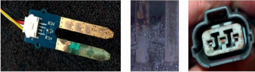
Fig. 3. Terminal corrosion caused by outgassed heat stabilizers or migration of other ionic impurities in the plastic (source: DSM)
