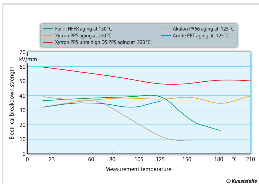
Fig. 8. Electric breakdown strength after aging at elevated temperatures. The curves of the materials are similar before and after aging. As a result of aging, the dielectric strength decreases as expected (source: DSM)
